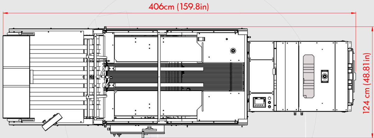
STP1000 AUTOMATIC FOLDING MACHINE
